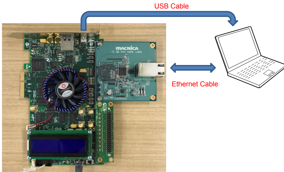
Figure 4-1 Connection Diagram for TI GE PHY HSMC CARD and evaluation computer.
