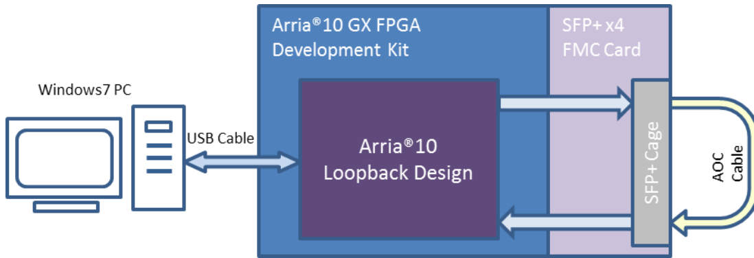
Figure 4-1 SFP+ x4 FMC Card Transceiver Toolkit Loopback Design Block Diagram
